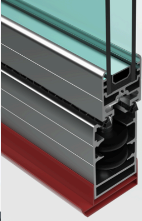
Damlalıklı alt kasa Bottom case with dropper
