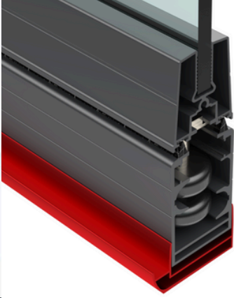
Damlalıklı alt kasa Bottom case with dropper
