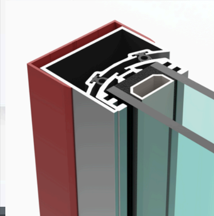
Ayarlı yan kasa Adjustable side frame
